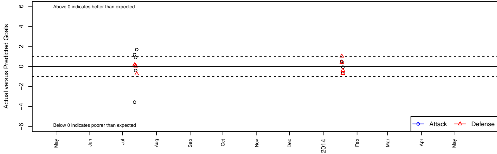
Leahi 01 Blue G00 Dots are actual minus expected GF (blue circles) and GA (red triangles). Blue line is smoothed change in attack strength. Red is smoothed change in defense strength.
